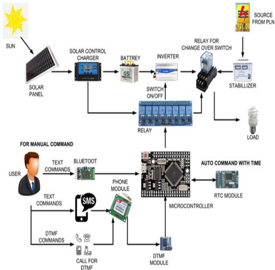
Figure 1. Chart of Smarthome Installation Implementation Based on Energy management
